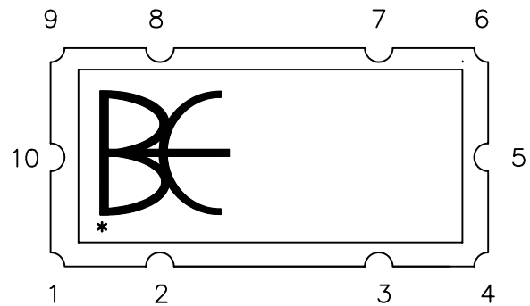
CONTACT I/O (TOP VIEW)
